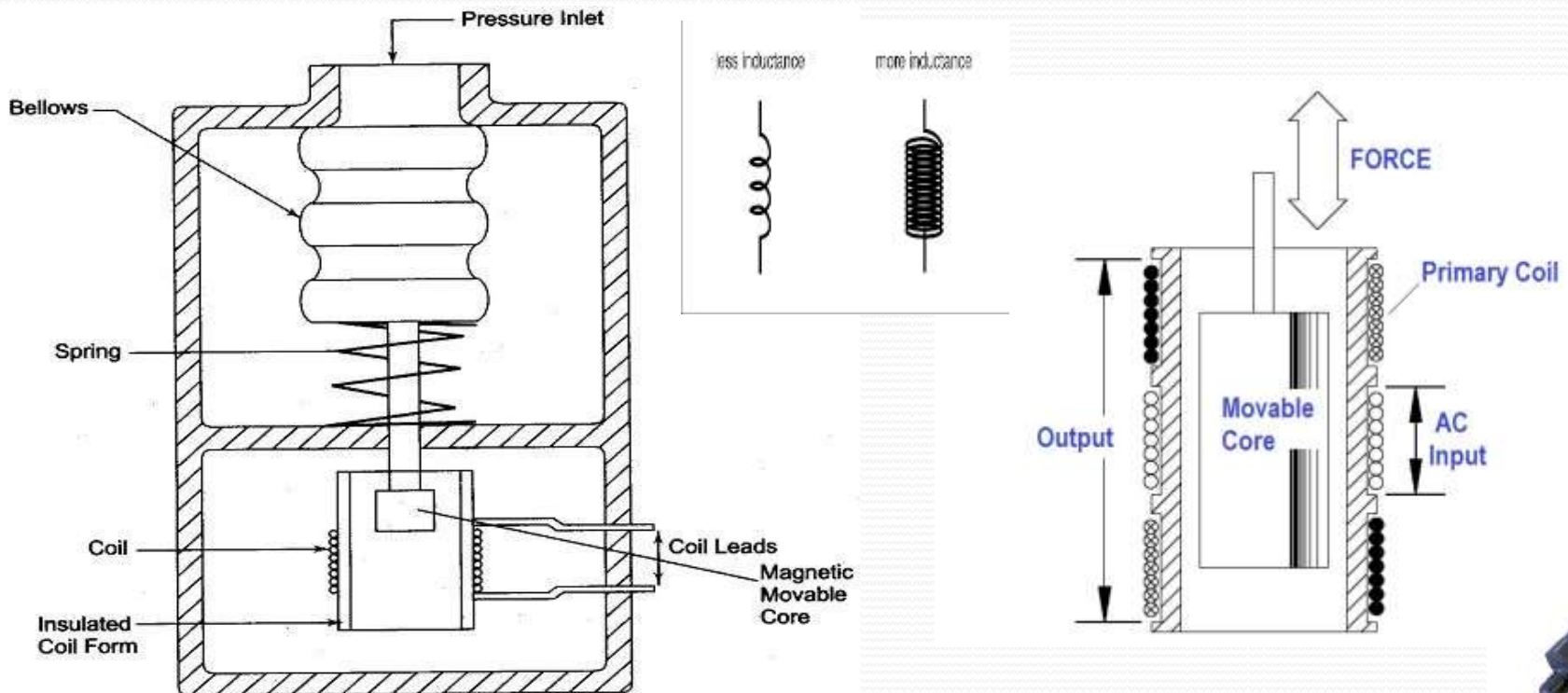
Fig. 13.22 Pressure Inductive Transducer
